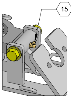
Alternate View of Yoke Assembly
