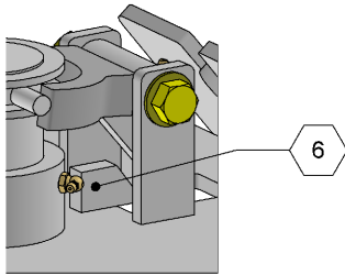
Alternate View of Air Pot Tab Stop
