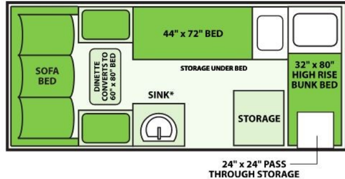
Floor Plan
