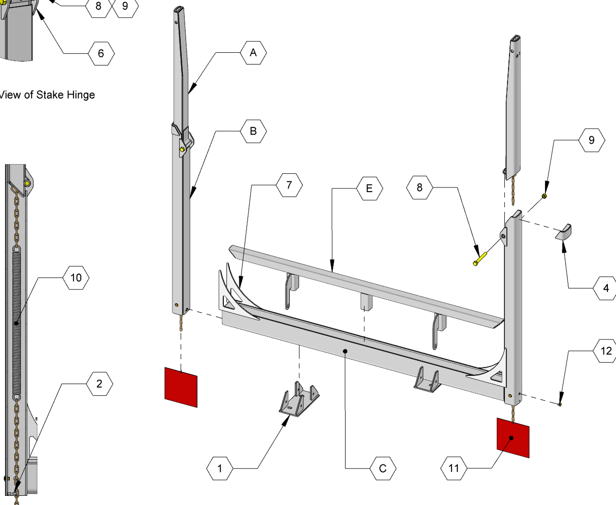
Section View of Main Stake
