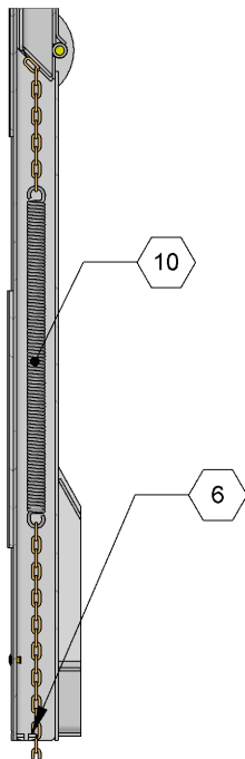
Section View of Main Stake
