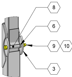
Detailed View of Stake Hinge
