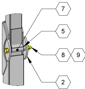
Detailed View of Stake Hinge
